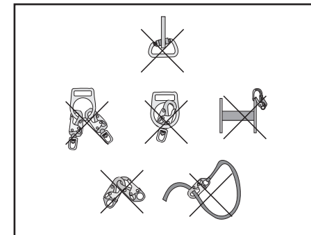
FIGURE 4 - INAPPROPRIATE CONNECTIONS
